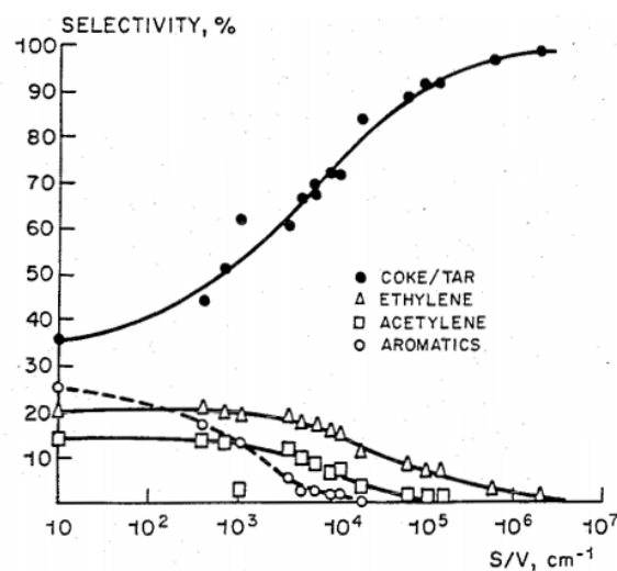
229 Figure 2. Selectivity to C_2H_4 , C_2H_2 , light aromatics and coke/tar as a function of surface to volume ratio at 25 %
