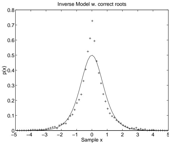
Figure 1: The sample histograms (marked +) of the deconvolved signals p(x) in case of unknown filter H_1(z) for the correct inverse model (left) and the inverse model with reflected roots (right) compared with the fixed model distribution \frac{1}{\cosh^2(x)} (solid line). Due to distribution mismatch the incorrect inverse filter (right) yields the global maximum of the joint entropy D(\vec{z}) .
