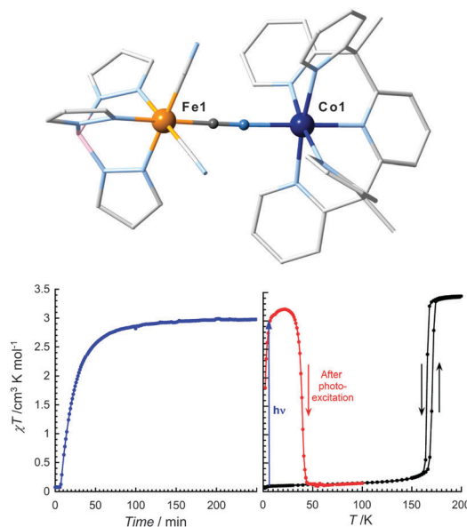
Fig. 8 (top) Representation of the molecular structure of [(\text{Tp})\text{Fe}(\text{CN})_3\text{Co}(\text{PY5Me}_2)](\text{OTf})\cdot 2\text{DMF} ( 27 ·2DMF) at T = 180 K. Hydrogen atoms, triflate and lattice-solvent molecules are omitted for clarity. Fe, Co, N and C atoms are indicated in orange, dark blue, light blue and light grey, respectively. (bottom) \chi T versus time (blue circles) of the desolvated compound, 27 , at 1 T and 10 K under white light irradiation ( 3 \text{ mW cm}^{-2} ), and \chi T versus temperature before (black dots) and after (red dots) white light irradiation with a sweep rate of 0.4 \text{ K min}^{-1} . Reprinted with permission from ref. 77. Copyright 2014 American Chemical Society.
