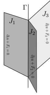
FIGURE 1. A parabolic equation posed on a multi-dimensional junction. Here there are 3 branches ( N = 3 ) and the tangential dimension is 1 ( d = 1 ). We did not illustrate the junction condition L = 0 on the junction hyperplane \Gamma (which is a line in this example).
