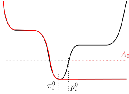
FIGURE 3. Non-increasing part H_i^- of a Hamiltonian H_i . The Hamiltonian is in black, the monotone part in red. The tangent variables (t, x', p') are not shown. In this example, the minimum of H_i is lower than A_0 .
