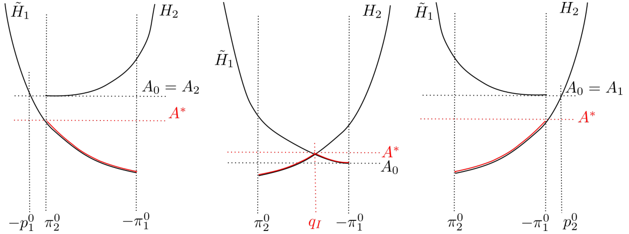
FIGURE 5. Three cases: Case 1 (left), Case 2 (center), Case 3 (right)
