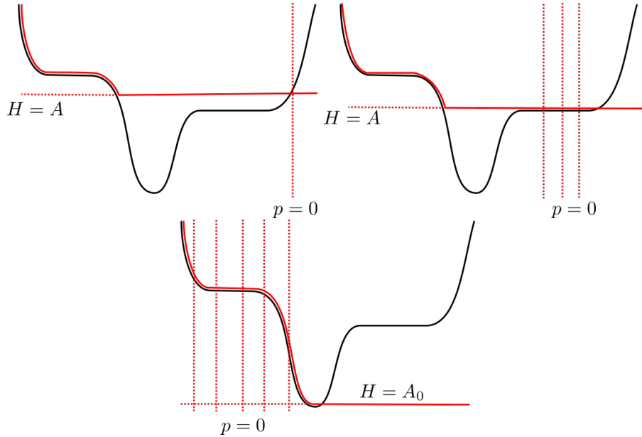
FIGURE 2. This figure illustrates Example 1.11 where N = 1 (number of branches) and d = 0 (dimension of the tangential space). The effective flux limiter A is determined in each case by looking at the points where the vertical line \{p = 0\} intersects the graph of the Hamiltonian H = H_1 ; the variable p reduces here to p_1 in the general setting.
