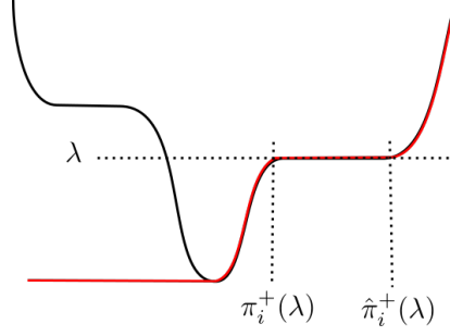
FIGURE 4. Non-decreasing part H_i^+ of a Hamiltonian H_i . The Hamiltonian is in black, the monotone part in red. The tangent variables (t, x', p') are not shown.
