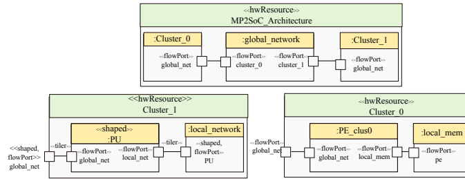
Fig. 7 UML/MARTE specification of the architecture
