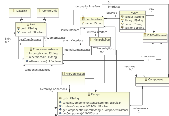
Fig. 2 S-LAM design meta-model
