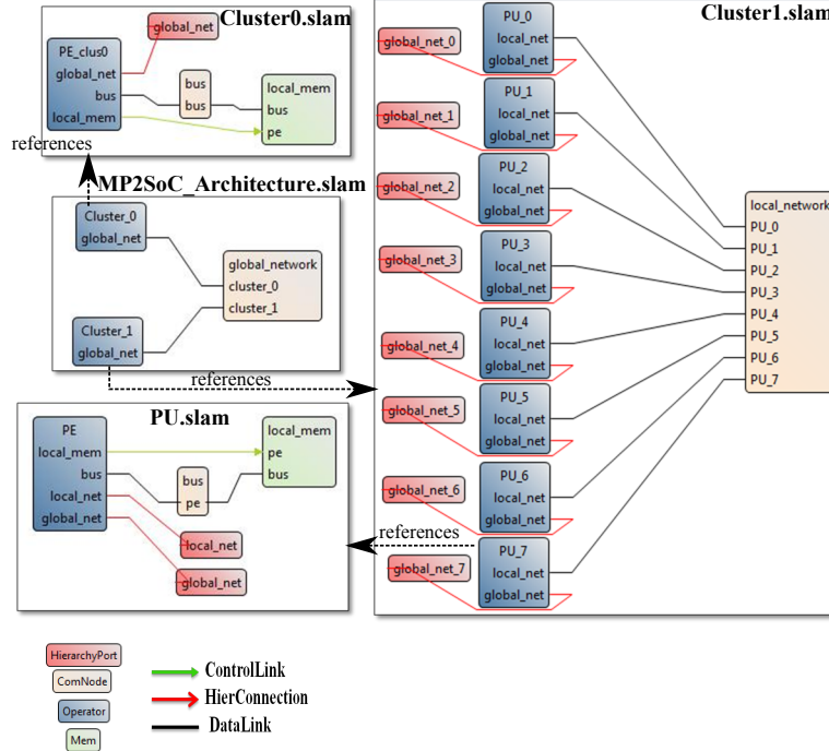
Fig. 8 Generated S-LAM files
