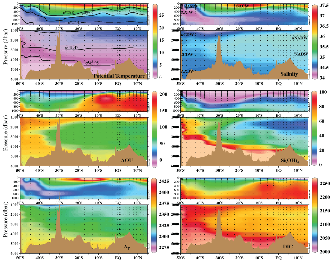
Figure 3. Section distributions of temperature (°C), salinity, AOU ( \mu\text{mol kg}^{-1} ), silicate ( \mu\text{mol kg}^{-1} ), A_T ( \mu\text{mol kg}^{-1} ) and DIC ( \mu\text{mol kg}^{-1} ) from the GEOTRACES-NL (2010/2011) data set.
