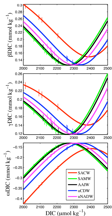
Figure 6. The buffer factors \beta\text{DIC} (top), \gamma\text{DIC} (middle) and \omega\text{DIC} (bottom) of each water mass over a range of DIC concentrations. The vertical lines denote the DIC concentration in pre-industrial times, 1994 and 2011 and the projected concentration in 2110.
