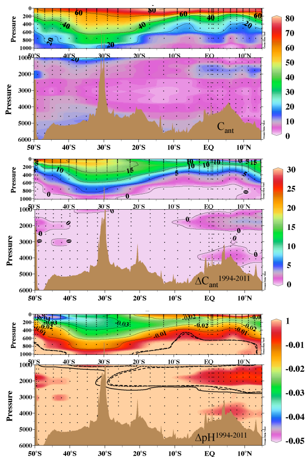
Figure 4. Distribution of C_{\text{ant}} ( \mu\text{mol kg}^{-1} ) calculated using the \phi C_T^0 method with the GEOTRACES-NL (2010/2011) data set (top); distribution of \Delta C_{\text{ant}}^{1994-2011} ( \mu\text{mol kg}^{-1} ), calculated using the eMLR approach (middle); and the distribution of the \Delta \text{pH}^{1994-2011} associated with \Delta C_{\text{ant}}^{1994-2011} (bottom). The aragonite saturation horizon ( \Omega \text{Ar} ) is marked for pre-industrial times (solid line), 1994 (dashed line) and 2011 (dotted line).
