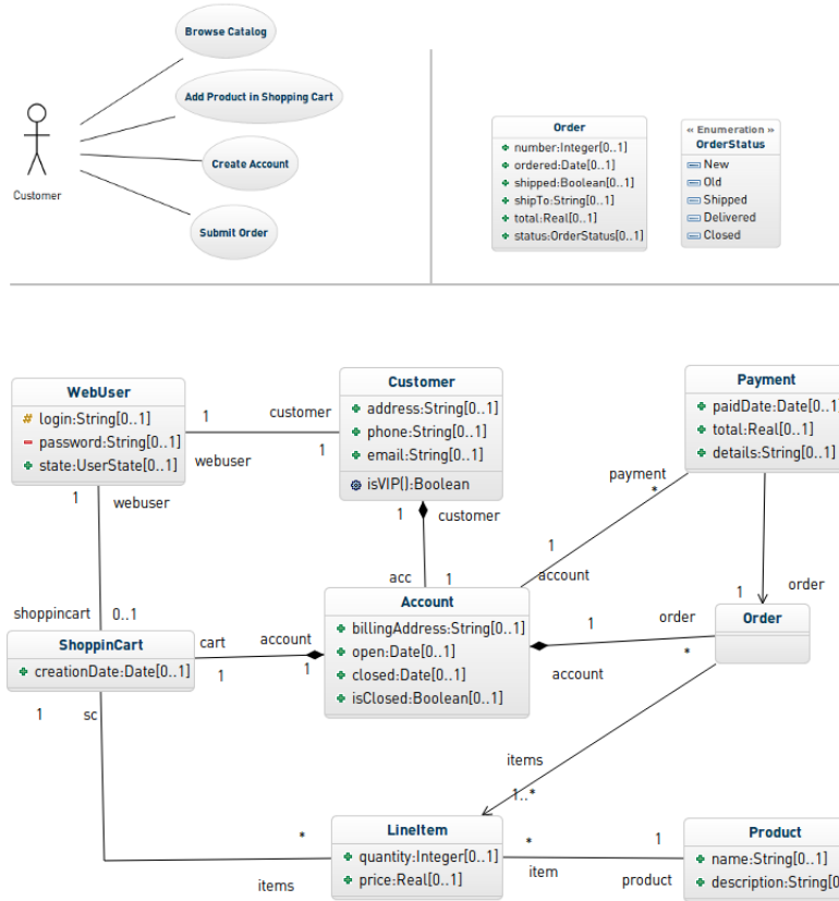
Fig. 2. Diagrams for webcomm model
