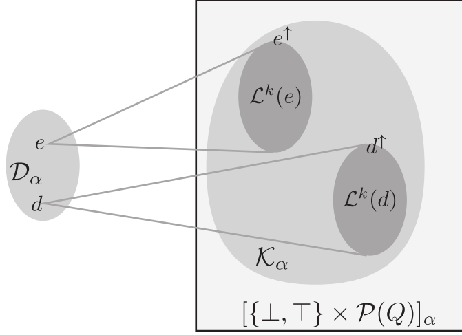
Figure 2: Model \mathcal{D} is embedded into model \mathcal{K} via logical relation \mathcal{L} .
