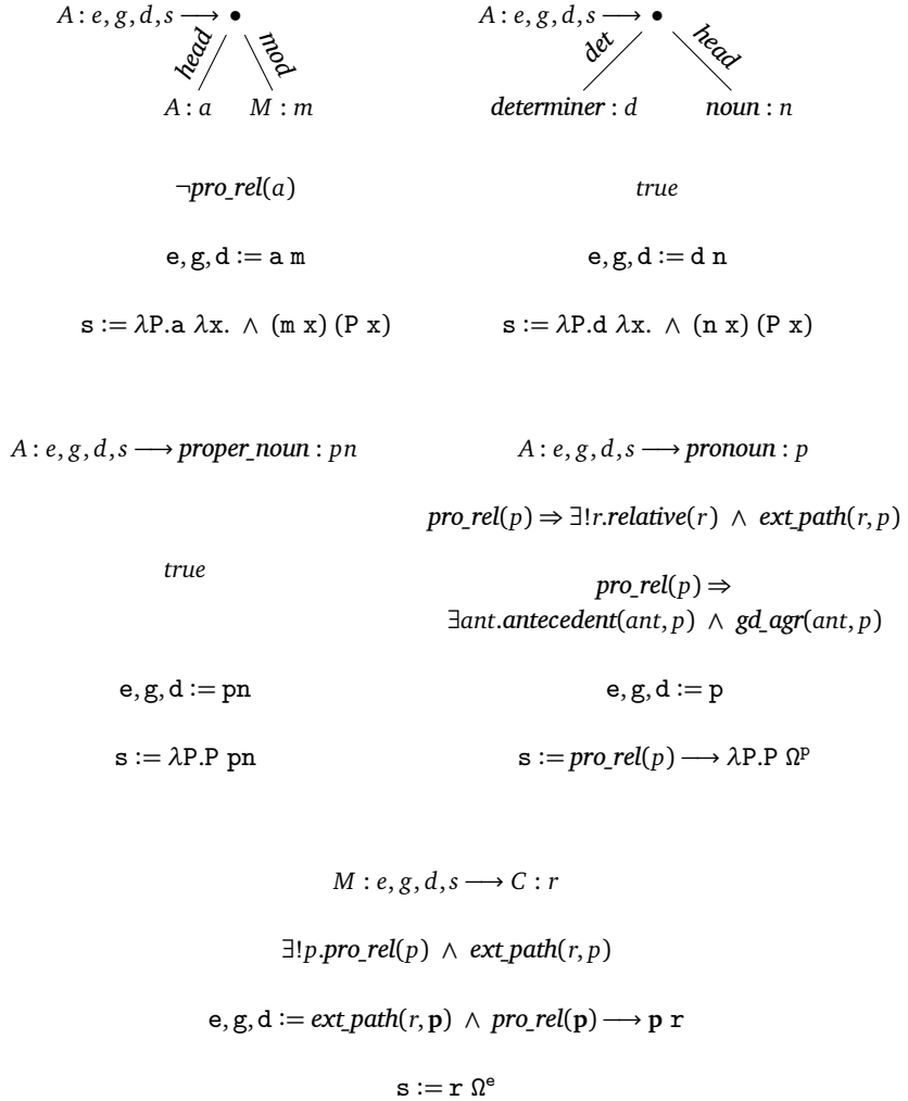
Figure 15: Second part of the full synchronous grammar, with logical constraints and linearizations
