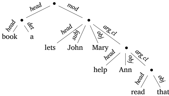
Figure 16: Abstract structure abs
