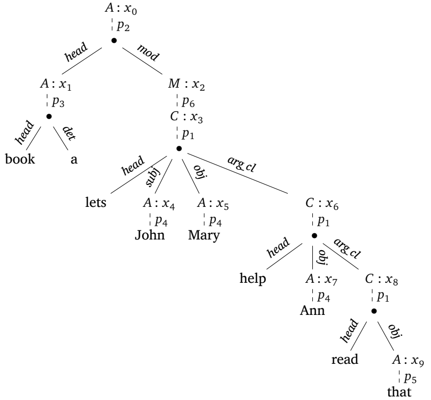
Figure 17: Derivation tree of abs
