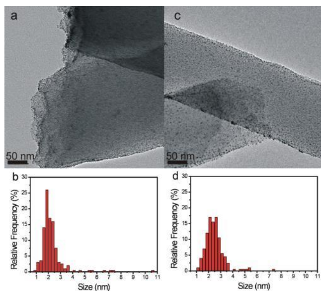
Figure 1. a, c) TEM images and b, d) particle distribution obtained from TEM analysis of a,b) Pt/CFs, c, d) SnO 2 /Pt/CFs before cyclic voltammetry.
