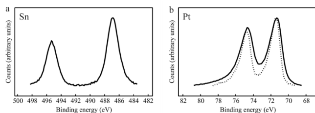
Figure 3. XPS spectra of SnO 2 /Pt/CFs (full line) and Pt/CFs (dotted line). High resolution scans across a) the Sn 3d and b) Pt 4f edges, respectively.
