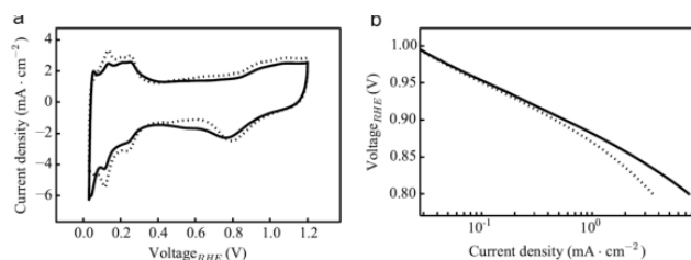
Figure 4. Cyclic voltammetry at 50 mV/s in a 0.5 M H 2 SO 4 solution saturated with N 2 . b) ORR Tafel plot for uncoated (dotted line) and SnO 2 -decorated carbon fibers (full line).
