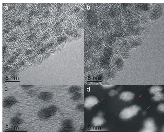
Figure 2. a, b HRTEM images of Pt/CFs and SnO 2 /Pt/CFs before cyclic voltammetry. c, d STEM images of SnO 2 /Pt/CFs in bright and dark field.
