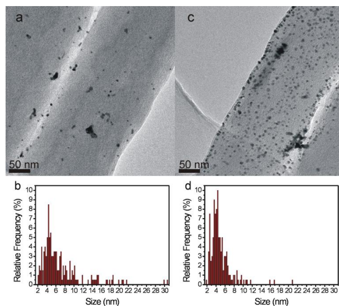
Figure 7. TEM images a,c) and b,d) particle distribution from TEM analysis of a,b) Pt 5% -CFs and c,d) SnO 2 -Pt 5% -CFs after 10,000 potential cycles.
