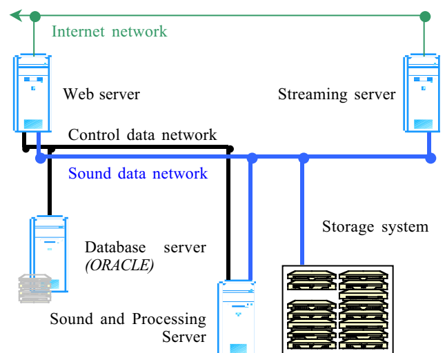
Figure 6. System architecture
