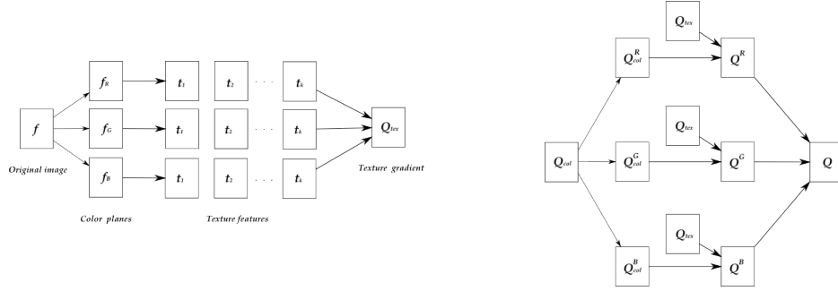
Fig. 1. Illustration of the structural gradient computation process (left: texture gradient computation; right: structural gradient computation).
