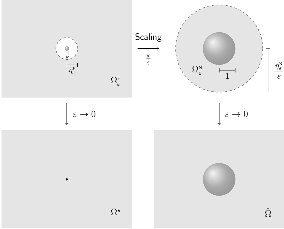
Figure 1: Far-field and near-field domains \Omega_\varepsilon^F and \Omega_\varepsilon^N and their limit \Omega^* and \hat{\Omega}
