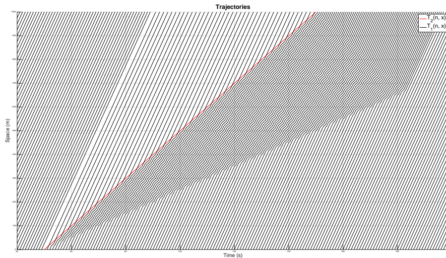
FIGURE 3 Impact of single slow vehicle (class 2) on fast vehicles (class 1)
