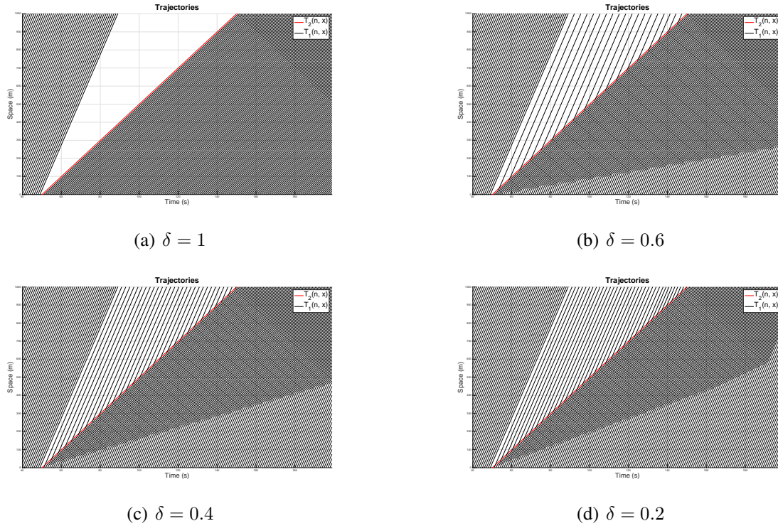
FIGURE 4 Impact of \delta on traffic states surrounding an active MB
