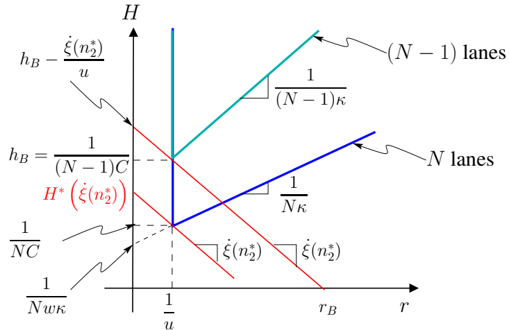
FIGURE 2 Moving bottleneck treatment in Lagrangian-space coordinates for a triangular Hamiltonian (for the sake of readability, the capacity drop is not represented here).
