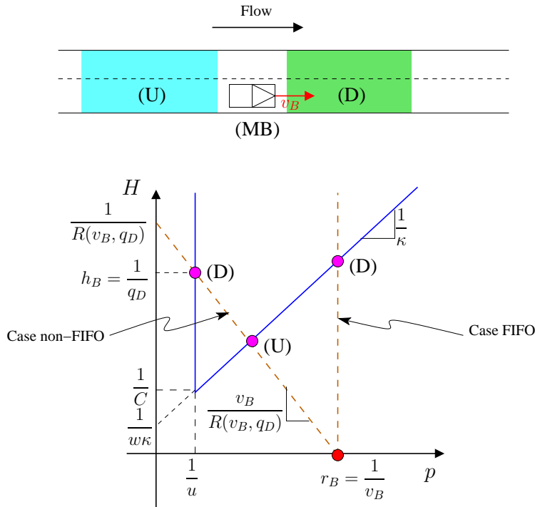
FIGURE 1 Moving bottleneck graphical solution in Lagrangian-space coordinates, for a triangular Hamiltonian, and with different values of the capacity drop parameter \delta .
