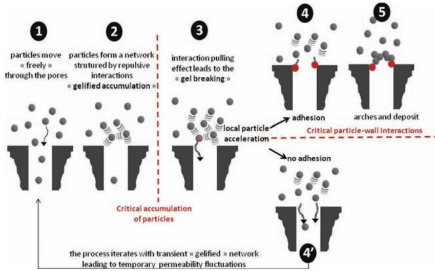
Fig. 16 Scenario for the mechanism of pore plugging with repulsive particles.
