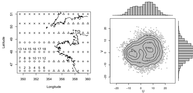
Figure 1. Left: Spatial hierarchical clustering of the moving variance associated with wind speed with four clusters (symbols). Right: Joint and marginal distribution of \{u_t, v_t\} at the central location 10; contour lines of the estimated joint density.
