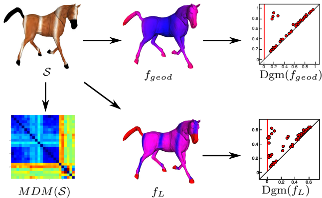
Fig. 6 Generating a PHOG signature. First row: A shape \mathcal{S} (left), the function f_{geod} (center) and the corresponding persistence diagram \text{Dgm}(f_{geod}) . Second row: the mutual distance matrix \text{MDM}(\mathcal{S}) , the function f_L and the corresponding persistence diagram \text{Dgm}(f_L) .
