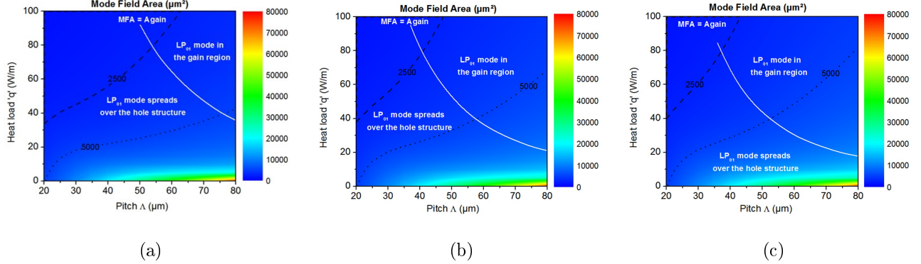
Figure 4. Evolution of the LP_{01} MFA with the heat load 'q' and the pitch \Lambda into (a) a 1 cell TGF, (b) 7 cells TGF and (c) 19 cells TGF. The white line depicts the limit when the MFA of the fundamental mode equals to the area of gain A_{gain} . Isolines also report MFA of 2,500 \mu m^2 (dashed line) and 5,000 \mu m^2 (dashed line).
