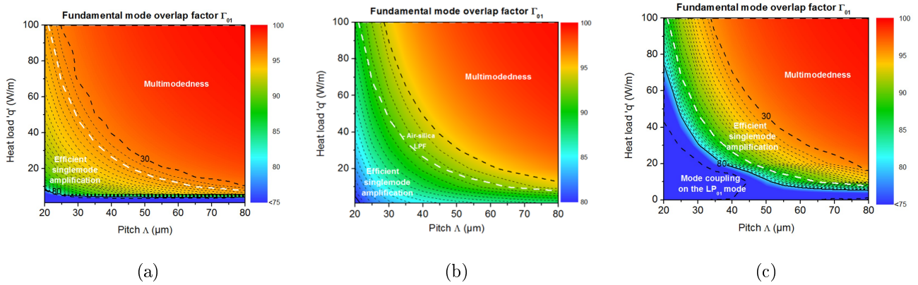
Figure 9. Evolution of the fundamental mode overlap factor with the heat load 'q' and the pitch \Lambda into a) a Symmetry-reduced PCF - d/\Lambda = 0.25 -, (b) an all-solid aperiodic LPF - d/\Lambda = 0.33 - and (c) an equivalent all-solid cladding reduced aperiodic LPF - d/\Lambda = 0.33 -. The thick solid/dashed black lines represent respectively the limit of each abovementioned criteria: an efficient amplification \Gamma_{01}=80\% and an effective singlemodedness criteria: \Delta\Gamma_{01}>80\% . The dashed area represents the region of efficient singlemode amplification and the thick dashed white line reports the upper limit of the singlemode range into a 19 cells air-silica LPF with d/\Lambda of 0.33.
