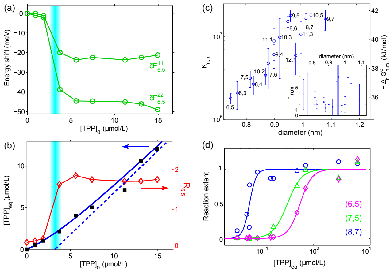
FIG. 3. (a) E^{11} and E^{22} energy shifts (green) as a function of the initial TPP concentration in a highly enriched (6,5) nanotube solution. (b) Free TPP equilibrium concentration (black squares) as a function of the initial TPP concentration, fit of TPP equilibrium concentration to the Hill equation (blue solid line) and its asymptotic form (dashed line); transfer ratio (red, see text) as a function of the initial TPP concentration. The light blue area shows the transition edge of the reaction. (c) Reaction constant (log scale) for several (n, m) nanotube species as a function of the diameter of the species as extracted from the fitting of the data shown in (d). Inset: corresponding Hill coefficients. (d) Functionalization extent as a function of the TPP equilibrium concentration (log scale) for selected species (symbols). Solid lines are fits of the Hill equation to these data.
