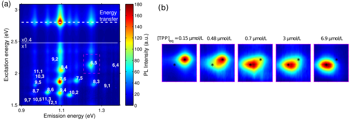
FIG. 2. (a) PLE map of a completely functionalized HiPCO solution. (b) Zoom on the region highlighted by a dashed red rectangle in (a) for selected TPP concentrations illustrating the evolution of the coverage of the (6,5) species. The black stars point at the shifted (resp. unshifted) position of the lines for a fully functionalized (resp. unfunctionalized) sample.
