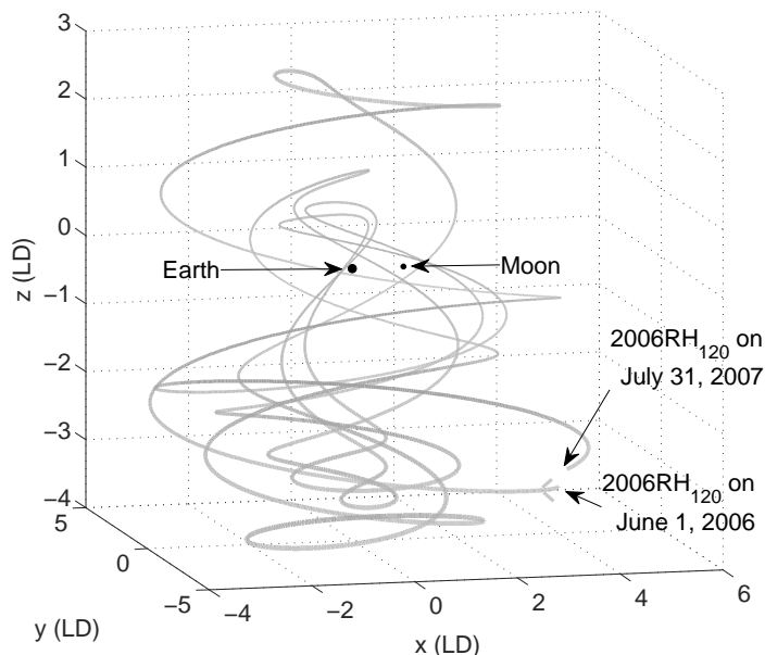
Figure 1: Orbit of RH_{120} in the Earth-Moon CR3BP rotating reference frame.
