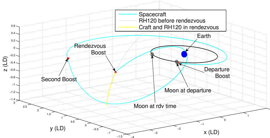
Figure 12: Best 3 boost Sun-perturbed rendezvous transfer to RH 120 from a Halo orbit around L_2 in inertial frame, with transfer departure after RH 120 detection.
