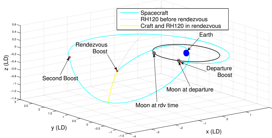
Figure 12: Best 3 boost Sun-perturbed rendezvous transfer to RH 120 from a Halo orbit around L_2 in inertial frame, with transfer departure after RH 120 detection.
