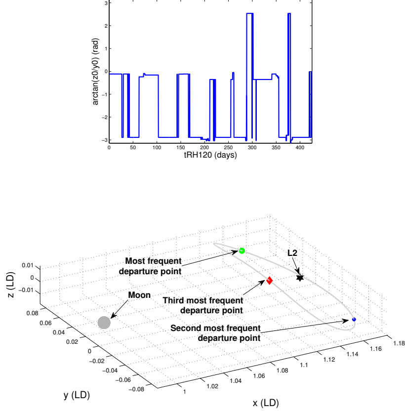
Figure 10: The top picture represents the evolution of (y, z)(0) argument with respect to time of rendezvous on RH_{120} . The bottom picture represents the three most frequent departure points on the initial Halo orbit.
