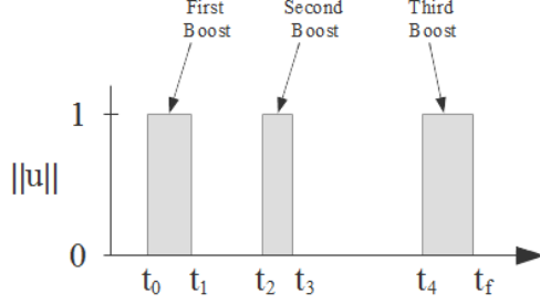
Figure 3: Control function modeling thrust impulses over time.
