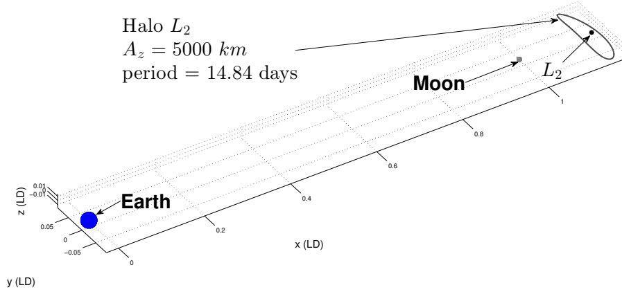
Figure 4: Halo orbit from which the spacecraft is departing, z -excursion of 5,000\text{ km} around the EM libration point L_2 .
