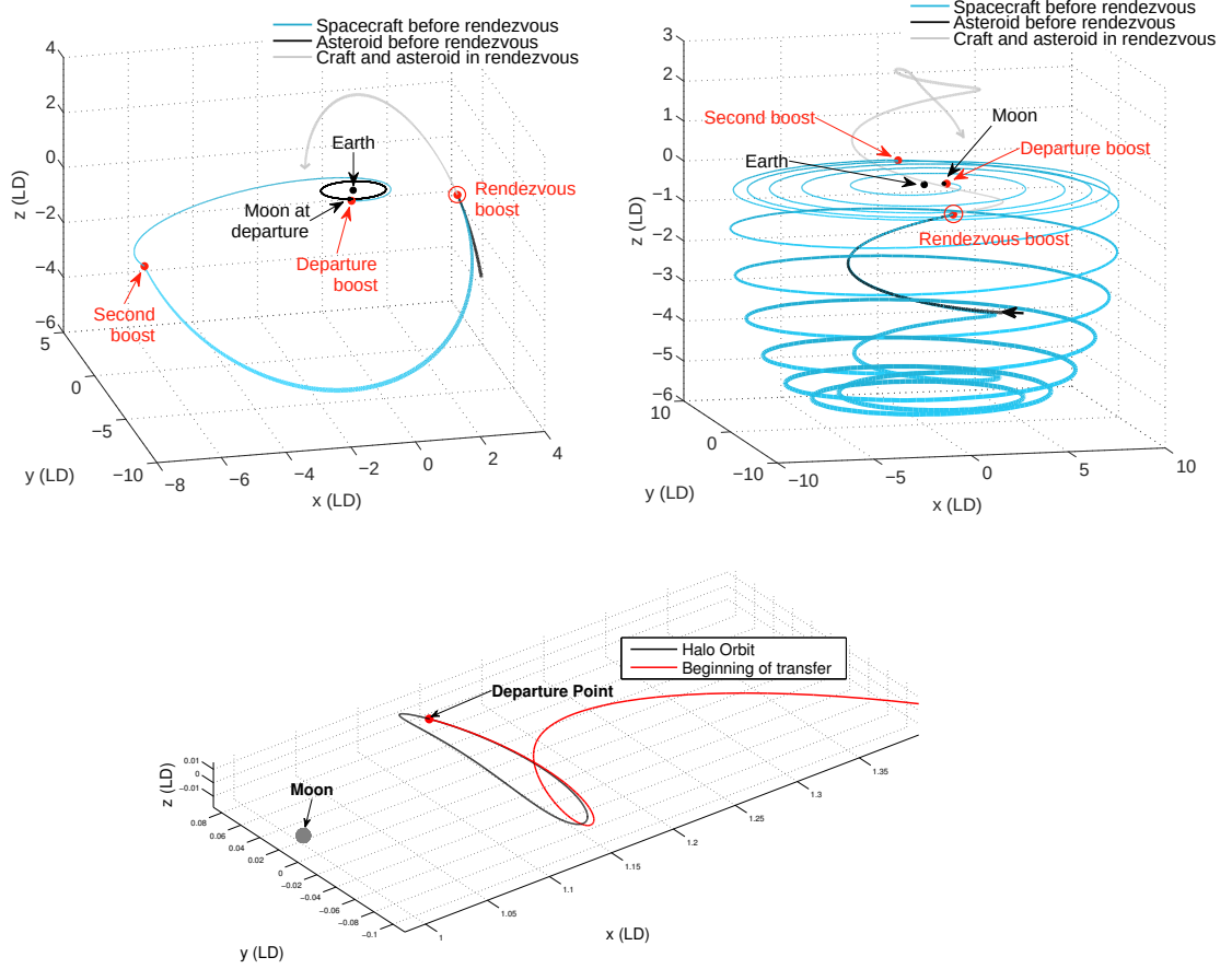
Figure 6: Best 3 boost rendezvous transfer to RH_{120} from a Halo orbit around L_2 : Inertial Frame (left). Rotating Frame (Right). Bottom: zoom on the start of the departure from the Halo orbit (rotating frame).
