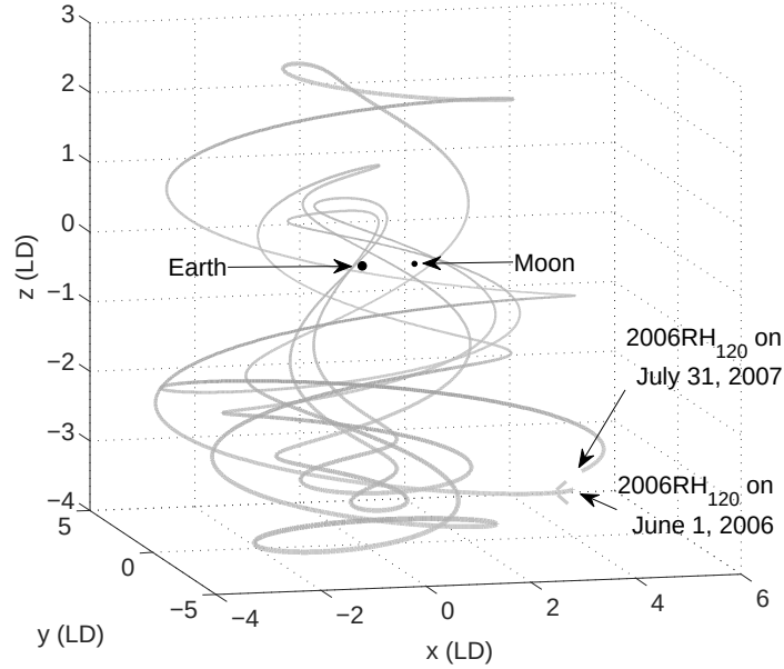
Figure 1: Orbit of \text{RH}_{120} in the Earth-Moon CR3BP rotating reference frame.
