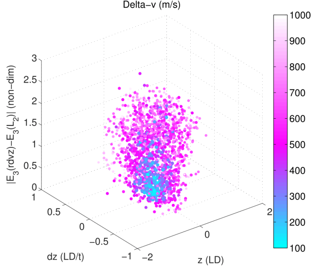
Figure 13: Characterization of 1,000 simulated rendezvous transfers from L_2 .
