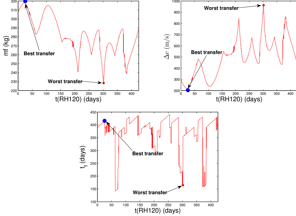
Figure 9: Evolution of the final mass (top left), of the \Delta v (top right) and transfer duration (bottom) from the Halo orbit around L_2 with respect to rendezvous points on the orbit of \text{RH}_{120} .
