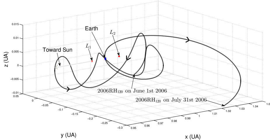
Figure 2: Orbit of RH_{120} in the Earth-Sun CR3BP rotating reference frame.
