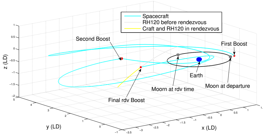
Figure 11: 3 boost rendezvous transfer to RH_{120} from a Halo orbit around L_2 in inertial frame, using the CR4BP. Departure 135 days after June 1 st 2006, arrival 255 days later.
