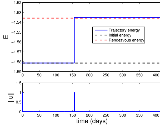
Figure 8: The bottom graph represents the control strategy for the best transfer to RH_{120} , and the top graph shows the evolution of the energy for this transfer. The energy of initial Halo orbit E_{HaloL2} = -1.581360 , the energy after 1st boost = -1.581335 , which means that the first boost raised the energy for about 2.46e-05 . The energy after 2nd boost = -1.535022 which is an increase of about 0.046313 and the energy at the rendezvous point = -1.535804 which is a decrease of about 7.814e-04 . The total energy difference is about 0.0456 .
