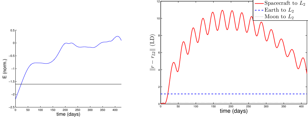
Figure 5: Evolution of the energy (left) and of the Euclidean distance to the L_2 Libration point (right) for RH_{120} . For energy, the horizontal line represents the energy of the Halo periodic orbit around L_2 which is about -1.58.
