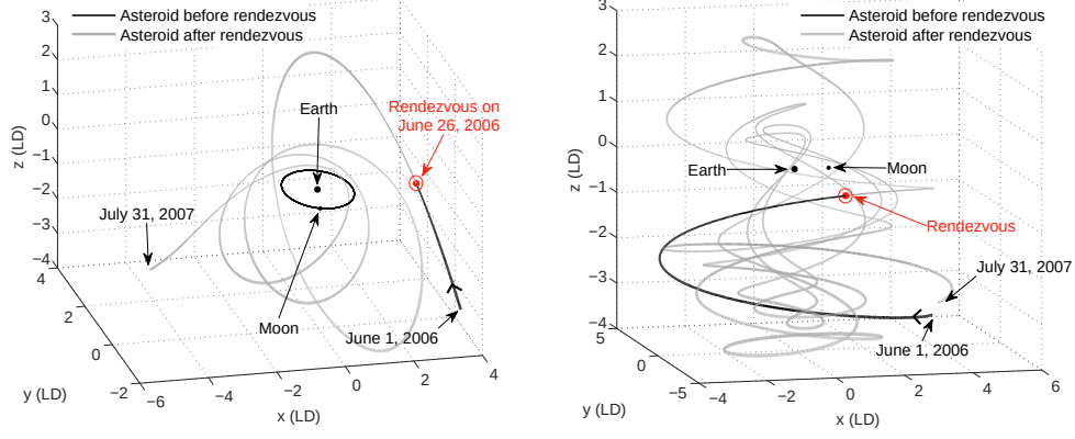
Figure 7: Best 3 boost rendezvous transfer to RH_{120} from a Halo orbit around L_2 : Inertial Frame (left). Rotating Frame (Right)
