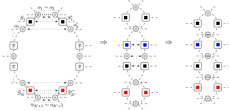
Figure 11: Left: two paths from the same outputs that form a simple cycle in g|g' . The pair of extremal inputs must be of a same color if a quotient whose \mathcal{GCC} is a tree exists. Such a quotient must be a quotient of the graph with identifications o_2 \sim o'_2 and o_Q \sim o_{Q'} , so we can iterate the reasoning.
