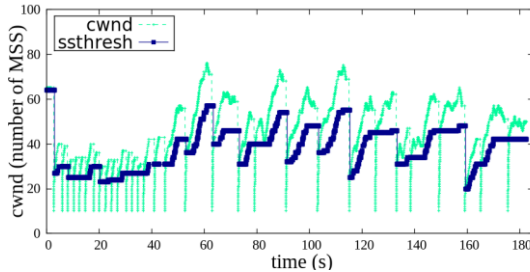
Figure 5. Cwnd variation of {Vegas, RTTM}
