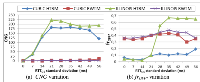
Figure 11. Variation of CNG and fr_{OFF^*}
