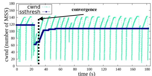
Figure 7. Cwnd variation of {Illinois RTTM},
