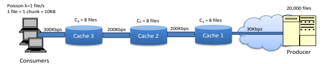
Fig. 1: Simulated line topology.
