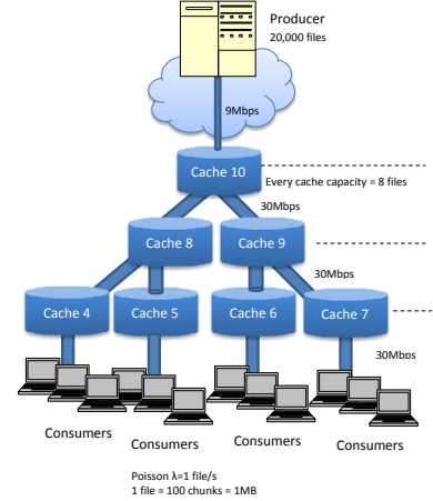
Fig. 3: Simulated tree topology
