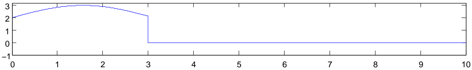
Repayment Density
