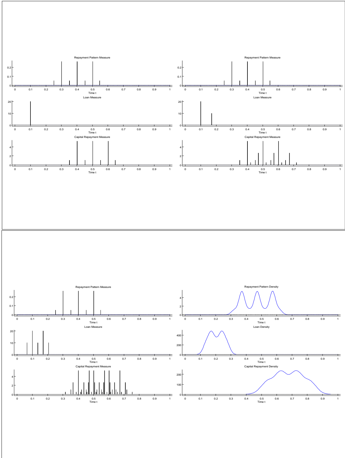
Figure 2: In each of the four pictures, \tilde{\gamma} is represented at the top, \tilde{\kappa}_E in the middle and \tilde{\rho}_K = \tilde{\kappa}_E \star \tilde{\gamma} at the bottom. These measures are concentrated measures in pictures at the left and in the top right picture. They are density measures in the bottom right picture.
