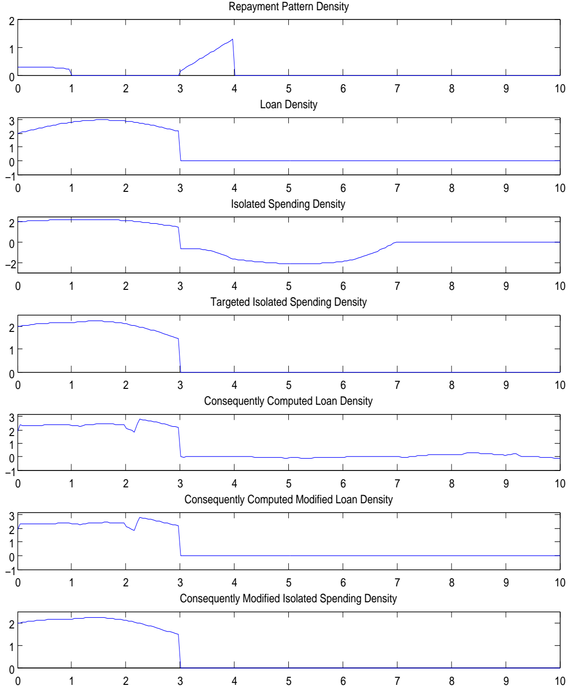
Figure 5: \tilde{\gamma} is represented in the top diagram, \tilde{\kappa}_E in the second diagram from the top, \tilde{\beta} in the third diagram from the top which is computed with relation (28) or (84), the fourth diagram from the top is targeted Isolated Spending Density, an new Loan Density is computed in the fifth diagram from the top, this density is modified to generate also a new Loan Density in the sixth diagram from the top, the bottom diagram is a consequently modified Isolated Spending Density which is same as \tilde{\beta} .
