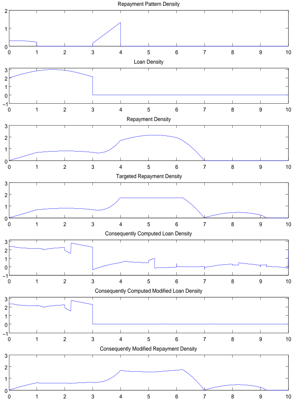
Figure 4: \tilde{\gamma} is represented in the top diagram, \tilde{\kappa}_E in the second diagram from the top, \tilde{\rho}_\kappa in the third diagram from the top which is computed with relation (7), the fourth diagram from the top is targeted Repayment Density which is supposed to be given, an new Loan Density is computed in the fifth diagram from the top, this density is modified to generate also a new Loan Density in the sixth diagram from the top, the bottom diagram is a consequently modified Repayment Density \tilde{\rho}_\kappa .
