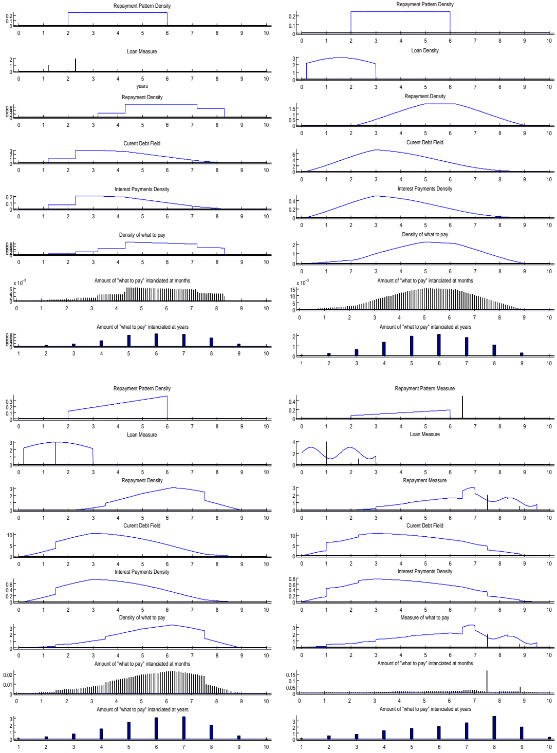
Figure 3: In each of the four pictures, \tilde{\gamma} is represented in the top diagram; \tilde{\kappa}_E in the second diagram from the top, \tilde{\rho}_K , which is computed with relation (7), in the third one; \mathcal{K}_{RD} which is computed according to relation (19) in the fourth one; \rho_I , calculated according to relation (10), in the fifth; the sixth diagram gives the density of what is to paid. The two last diagrams are respectively the amounts of what to pay over monthly and yearly period.
