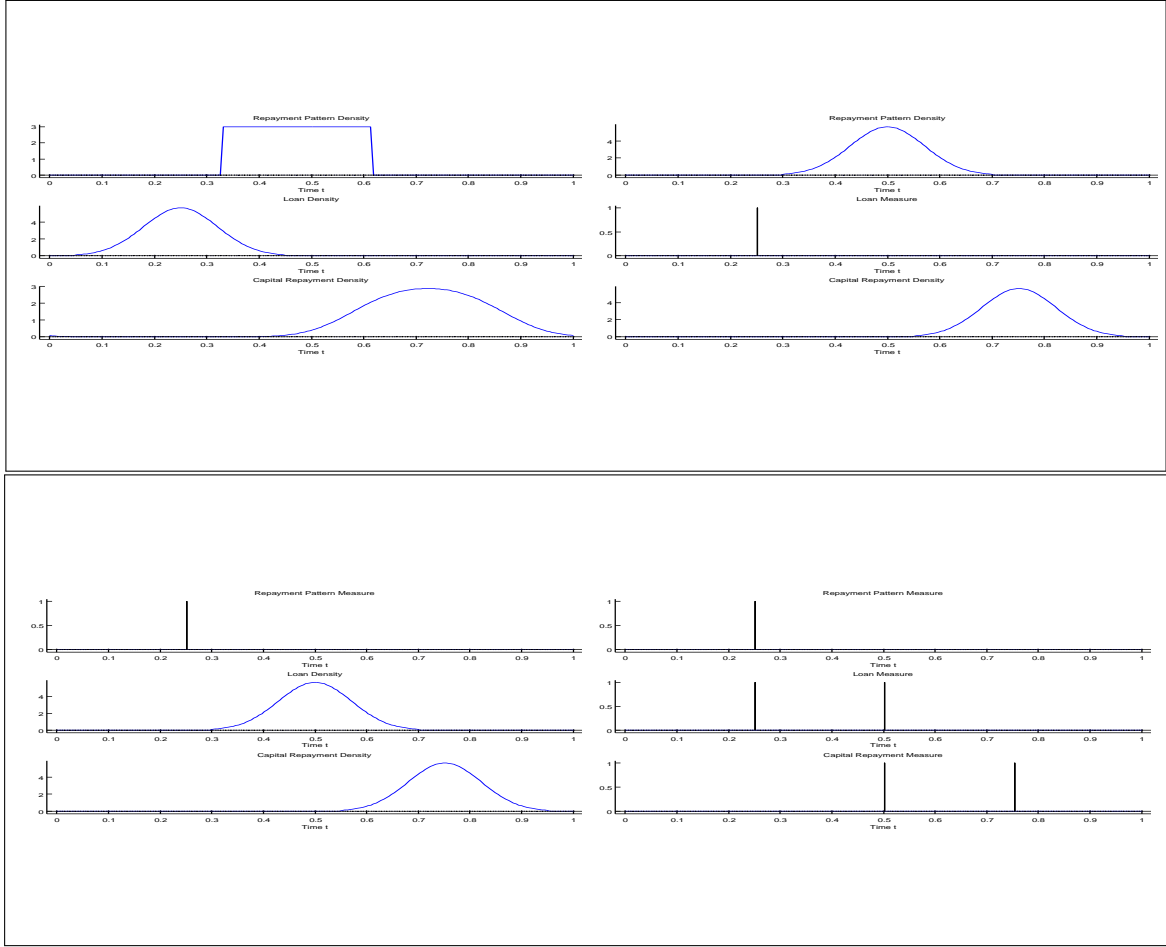
Figure 1: In each of the four pictures, \tilde{\gamma} is represented at the top, \tilde{\kappa}_E in the middle and \tilde{\rho}_K = \tilde{\kappa}_E \star \tilde{\gamma} at the bottom. (When the considered measure is a density measure, its density is drawn. When it undergoes concentrations, bars located at the concentration positions, with height the amount which is concentrated at each location, are drawn).
