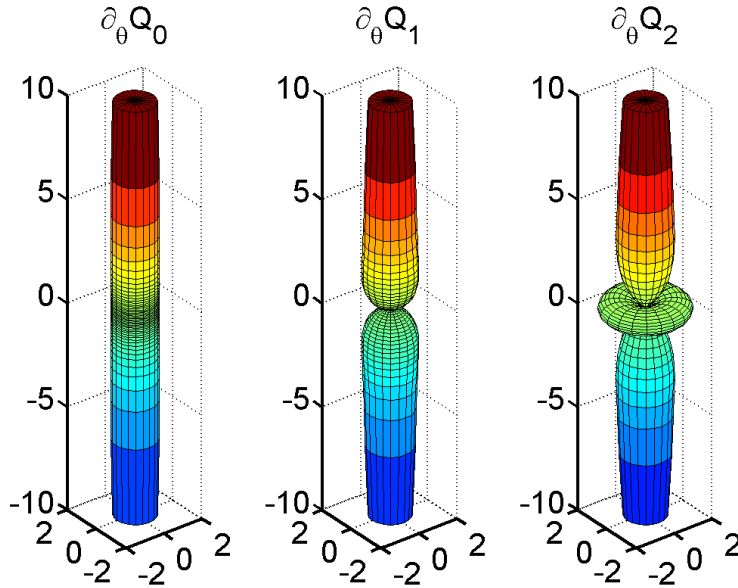
Figure 8: Derivative of the Legendre functions of the second kind Q_0 , Q_1 and Q_2 . The surface plot is given by \partial_\theta Q_l(\cos\theta) \vec{e}_r and have been truncated for \partial_\theta Q_l(\cos\theta) > 10 since they diverge at \theta = 0 and \theta = \pi .
