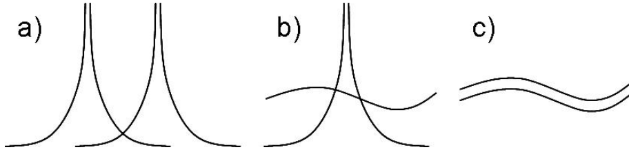
Figure 2: Schematic representation of particle interactions: “near field” fermion-fermion interaction (a), fermion-boson or “far-field” fermion-fermion interaction (b) and boson-bosons interaction (c). “Near field” and “far-field” have to be understood as in standard optics by comparing distances to the wavelength.
