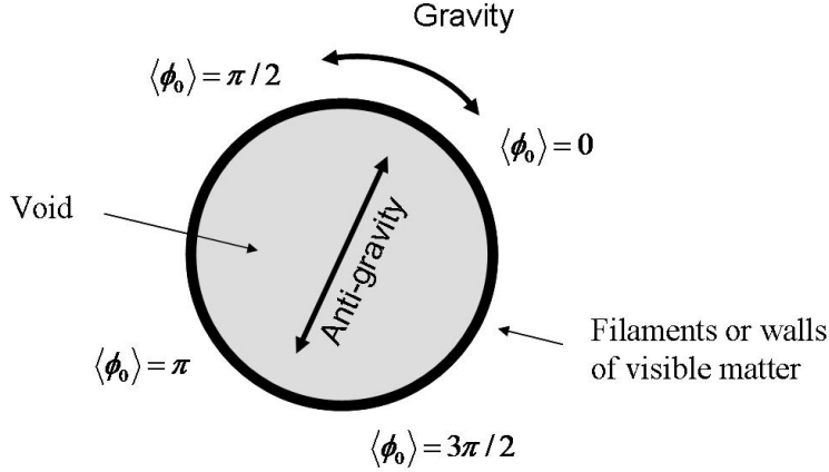
Figure 9: Large scale structures in universe including here filaments, walls and a single void. The average phase of matter varies continuously from \phi_0 = 0 [2 \pi ] to 2\pi [2 \pi ] along the filaments or walls.
