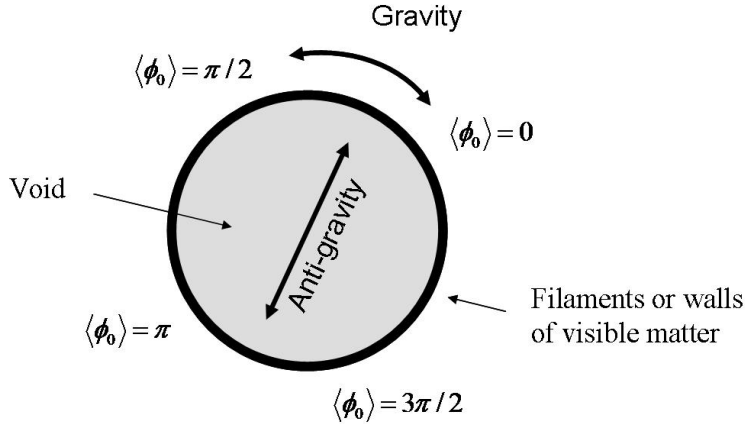
Figure 9: Large scale structures in universe including here filaments, walls and a single void. The average phase of matter varies continuously from \phi_0 = 0 [2 \pi ] to 2 \pi [2 \pi ] along the filaments or walls.
