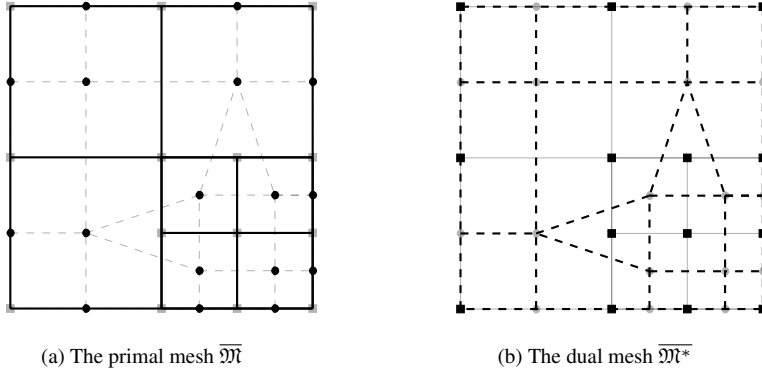
Fig. 2.2: A DDFV mesh \mathcal{T} made of non-conforming quadrangles
