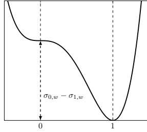
Fig. 1.3: Degenerate double-well structure of f_s
