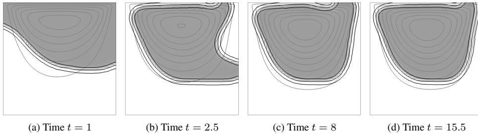
Fig. 5.5: Solution for \theta_s = \frac{\pi}{3}
