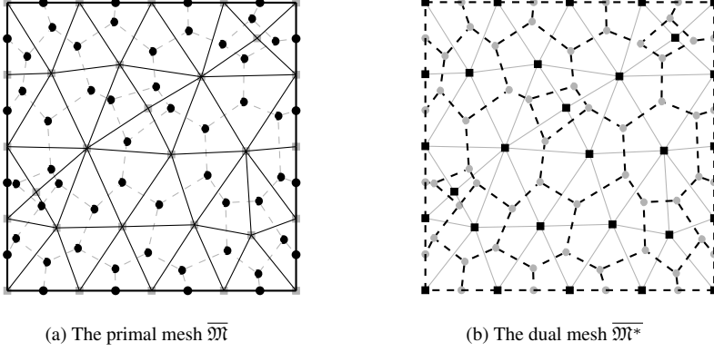
Fig. 2.1: A DDFV mesh \mathcal{T} made of conforming triangles
