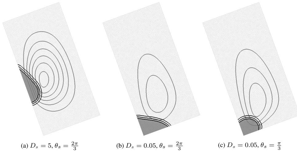
Fig. 5.2: Solution at time t = 10
