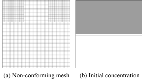
Fig. 5.3: Primal mesh \mathfrak{M} and initial data
