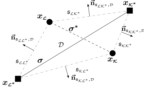
Fig. 4.1: Definitions in a diamond cell \mathcal{D} \in \mathcal{D}
