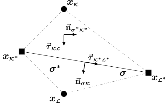
Fig. 2.3: Notations in a diamond cell \mathcal{D}
