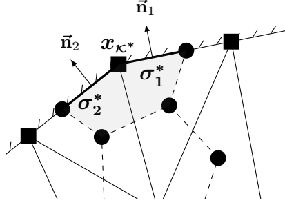
Fig. 2.4: Case where x_{\kappa^*} is a corner point of \Omega
