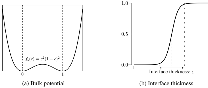
Fig. 1.1: Double-well structure of f_b and definition of the interface thickness
