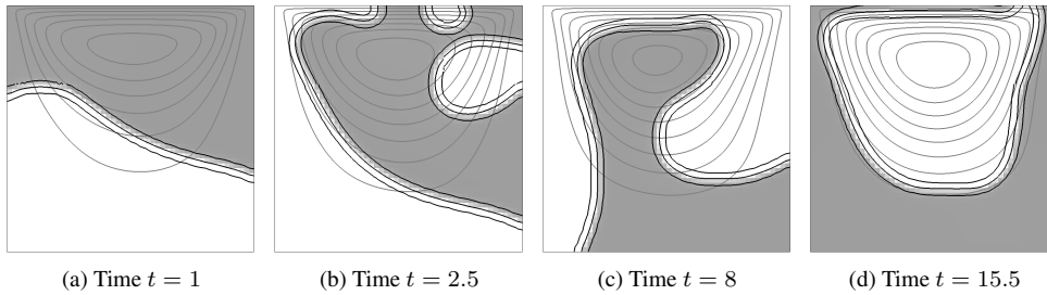
Fig. 5.4: Solution for \theta_s = \frac{2\pi}{3}
