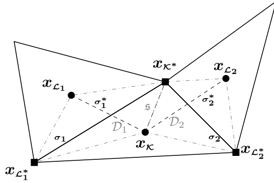
Fig. 4.2: Notations for the construction of \mathcal{G}^\mathcal{T}
