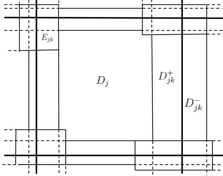
Figure 1: Schematic view of the decomposition of the control volume
