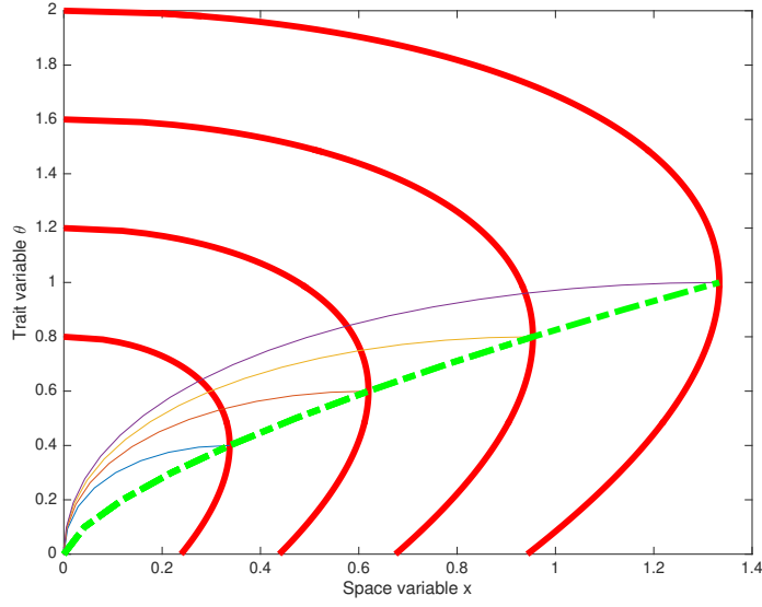
Figure 2.1: The level set \{\bar{u}(t, x, \theta) = 1\} in the phase space (x, \theta) for different values of time and the optimal trajectory, see also [11]. We also plot the trajectories that lead to the edge of the front for various values of time. These latter trajectories are crucial for the paper.
