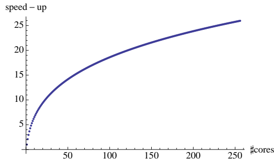
Fig. 5 Predicted speed-up in case of a lognormal distribution, with x_0 = 0 , \mu = 5 and \sigma = 1 , w.r.t. the number of processors.
