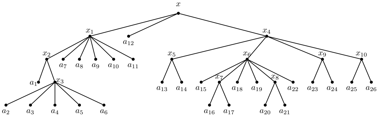
Figure 4.1: The tree t(x) .
