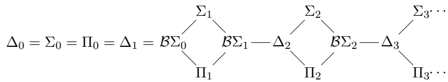
Figure 10.3: The logical hierarchy
