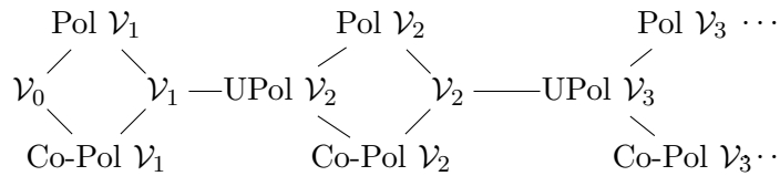
Figure 10.4: The Straubing-Thérien hierarchy
