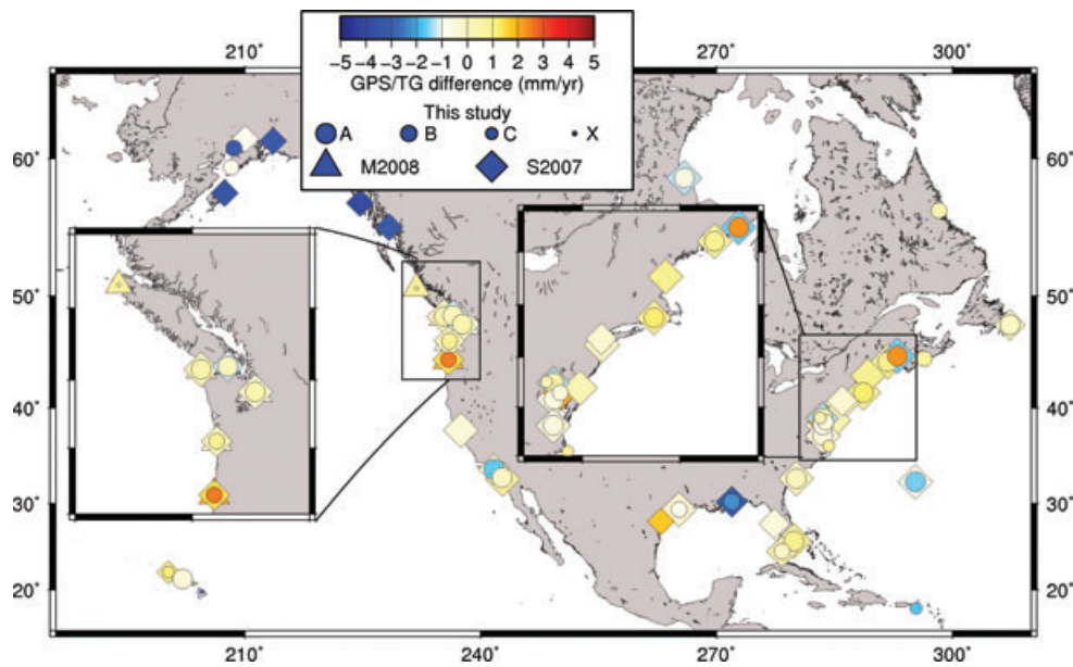
Figure 5. Map of the differences between the GPS and TG velocities in North America, in \text{mm yr}^{-1} : this study (circle with size corresponding to the station groups; A represents the pairs of stations of best quality, X the poorest ones); Mazzotti et al. (2008) (M2008, triangles); and Snay et al. (2007) (S2007, diamonds). Enclosed are two insets showing in more details the west and east coast stations.
