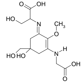
Shinorine
