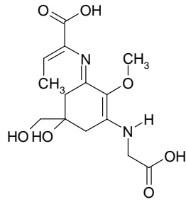
Palythenic acid
