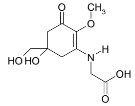
Mycosporine-glycine
