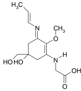
Palythene
