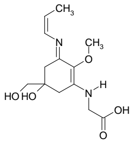
Usujirene
