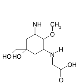
Palythine
