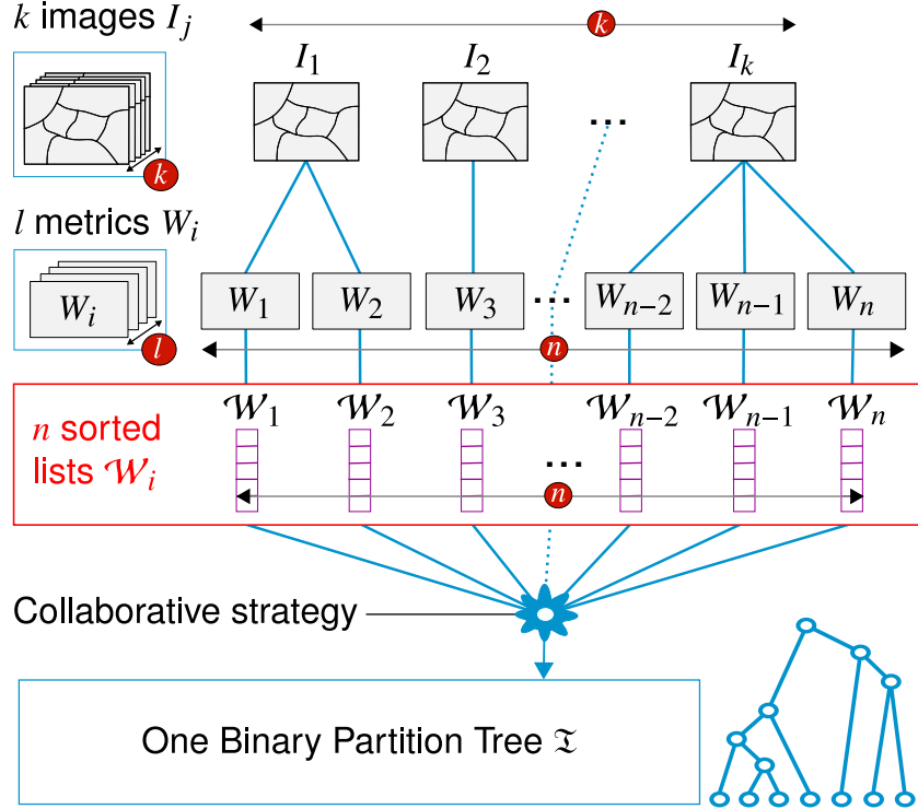
Figure 3: General structure of a BPT creation involving n valuation functions / sorted lists. Each list \mathcal{W}_i gathers edges information computed by using one valuation function corresponding to a given metric on an image. A BPT is obtained by applying a collaborative strategy leading to a consensus between the information carried by these n lists (see Section 4.2).
