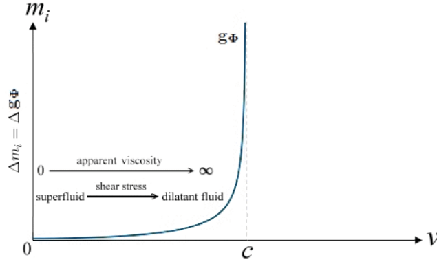
Figure 4: relativistic mass increase, where \Delta m_i corresponds to \Delta g_{\Phi} . This graph can also be interpreted as a rheogram of quantum space. As shear rates and flow velocities move toward relativistic values, collisions among SQ intensify and viscosities, albeit initially near zero, critically increase.
