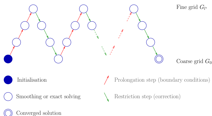
FIGURE 2 – Representation of the iterative process in \Lambda -cycle meshes
