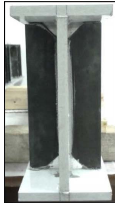
Fig. 2b. Type 2 beam – photo.
