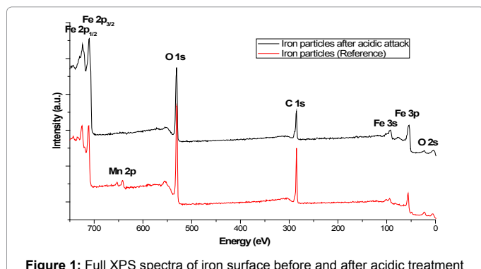
Figure 1: Full XPS spectra of iron surface before and after acidic treatment
