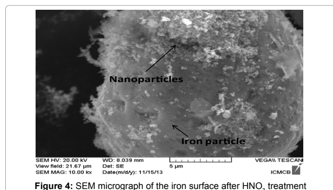
Figure 4: SEM micrograph of the iron surface after HNO 3 treatment
