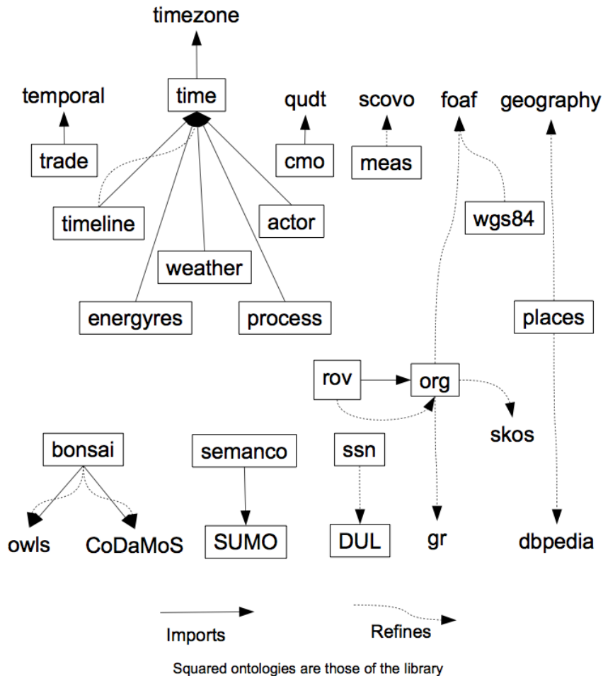
Figure 26. Relations between the 16 ontologies which import or refine others. At the bottom of the picture are general ontologies and at the top specialized ontologies.
