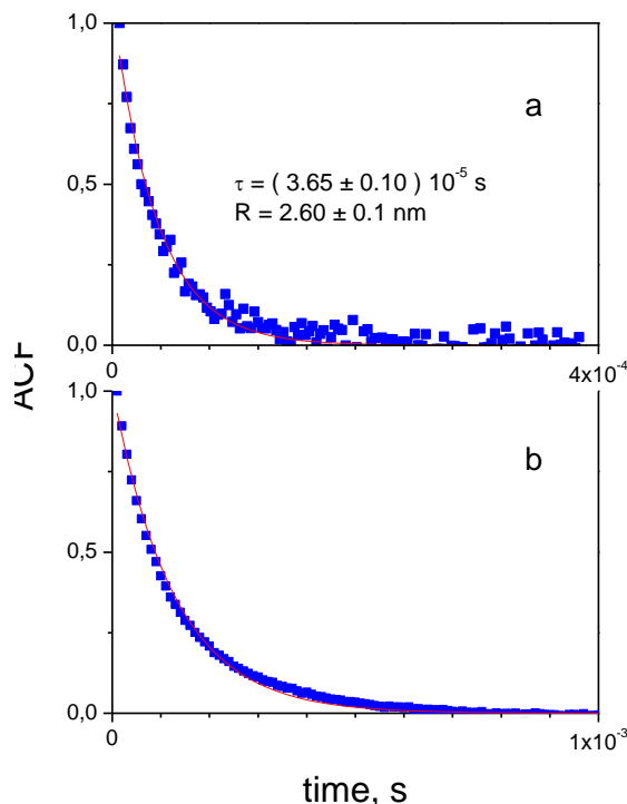
Figure 2: Characteristic ACFs of oxo- \text{TiO}_2 nanoparticles after preparation in the sol-gel reactor ( [\text{Ti}] = 0.15 \text{ M} , H = 2 , T = 20^\circ \text{C} , 2-propanol solution) (a) and after surface exchange with MAPTMS ( C_{\text{Ti}} = 1.5 \text{ M} ) (b).
