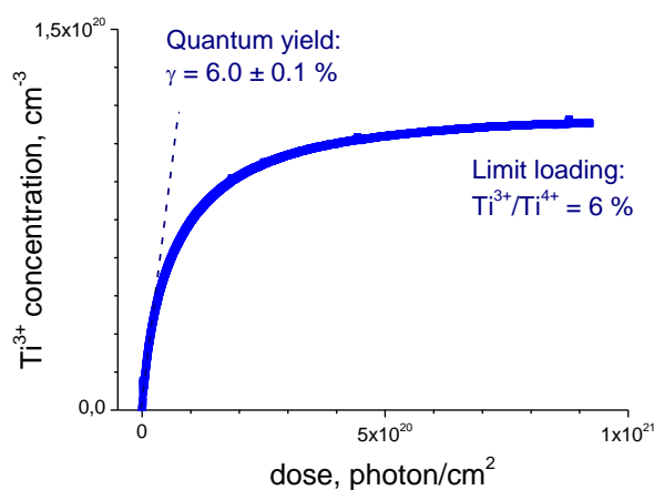
Figure 5 : Darkening kinetics of MAPTMS-TiO 2 hybrids ( C_{Ti} = 3.0 M or 1.8 \cdot 10^{21} cm^{-3} , sample thickness 93 \mu m ).
