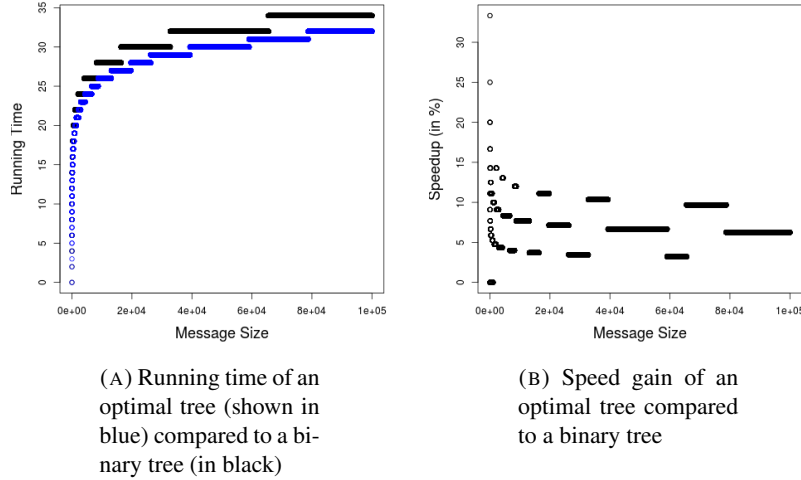
FIGURE 3. Performance comparison between an optimal tree and a binary tree
