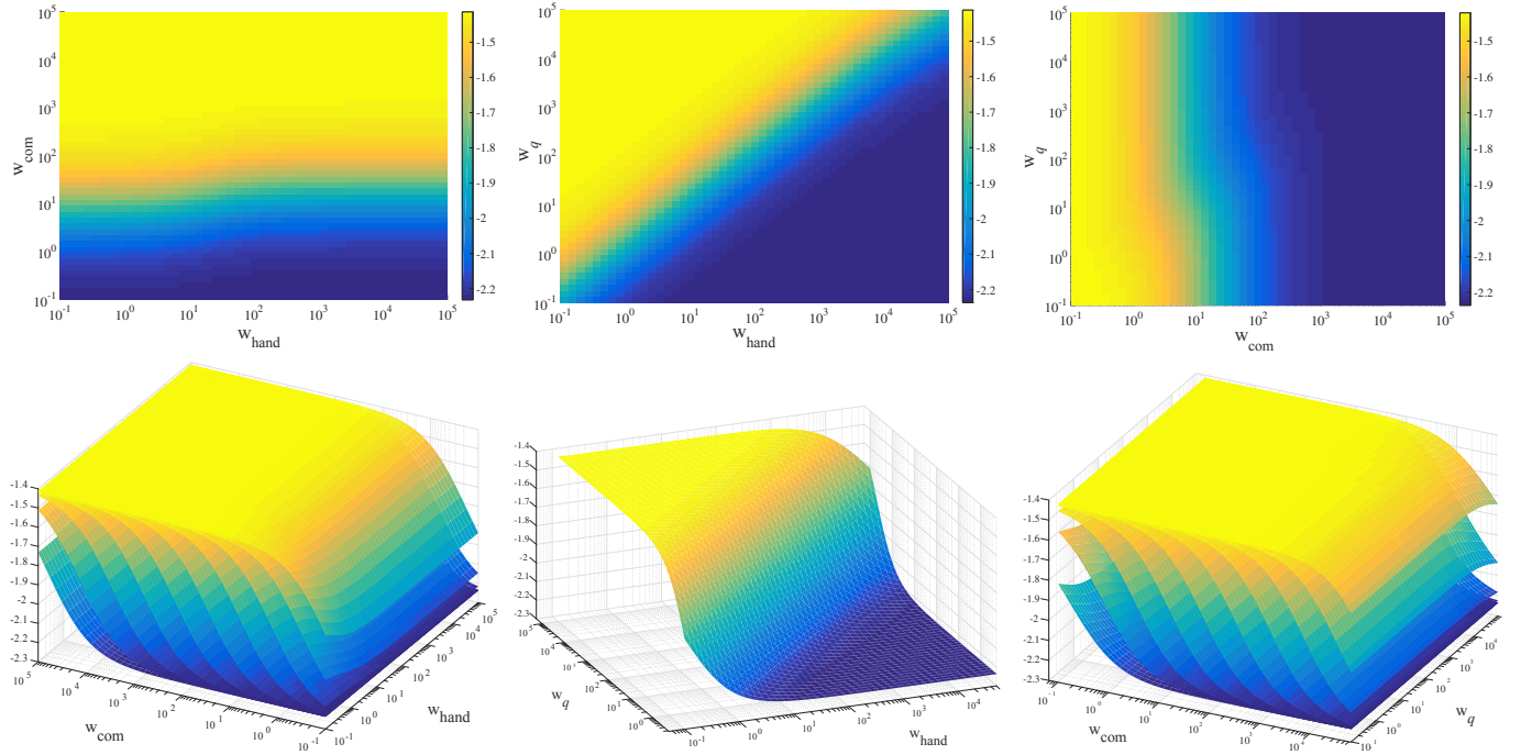
Fig. 5. Matrix stability from Proposition 4. We discretized the (w_{hand}, w_{com}, w_q) space in 50 \times 50 \times 50 grid in logarithmic scale ranging from 10^{-1} to 10^5 along each dimension of the weight vector (w_{hand}, w_{com}, w_q) \in \text{logspace}(-1, 5, 50)^3 . We plot in color scale and surface plot the maximum real part of the eigenvalues of the matrix from Proposition 4. We see that this maximum is always negative, hence the matrices are stable. In the top row figures we plot the maximum real part of the eigenvalues along two dimensions of the weight vector for a given value of the third dimension ( 10^4 ). In the bottom row figures we plot the same data for 10 values in \text{logspace}(-1, 5, 10) along the third dimension while the other two dimensions are in \text{logspace}(-1, 5, 50)^2 which result in 10 surfaces in each plot (the 10 surfaces are very close to each other in the middle column).
