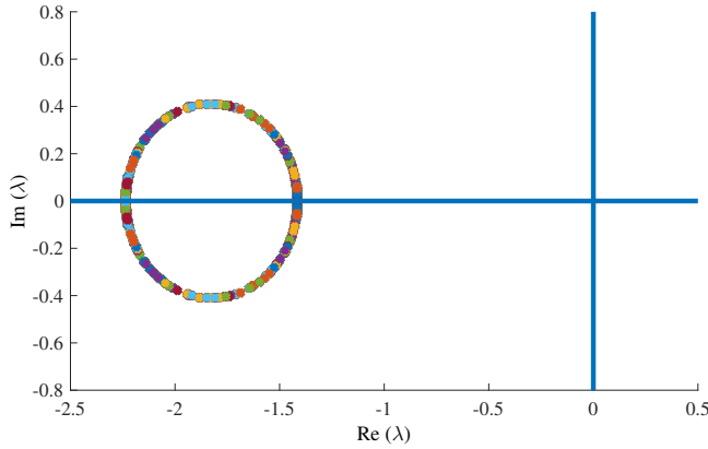
Fig. 6. All 112000 eigenvalues (counting multiplicities) of the 112x112 matrices from Proposition 4 for 1000 set of weights ranging in logarithmic scale from 10^{-1} to 10^5 , i.e. (w_{hand}, w_{com}, w_q) \in \text{logspace}(-1, 5, 10)^3 . All the eigenvalues are located in the left complex half plane which means they are stable.
