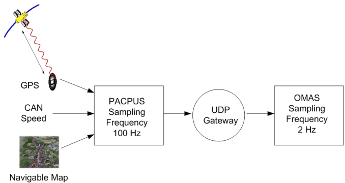
Figure 12. UDP connection between PACPUS and OMAS
