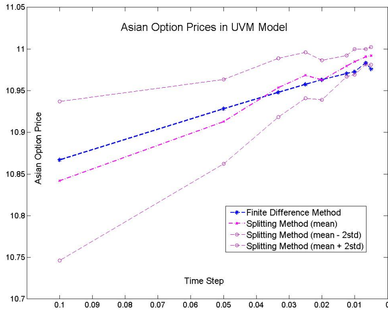
Figure 1: The comparison of some numerical methods for pricing Asian option with payoff (A - K_1)^+ - (A - K_2)^+ in UVM, with parameters S_0 = 100 , K_1 = 90 , K_2 = 110 , T = 1 , r = 0.05 , \sigma = 0.18 , \bar{\sigma} = 0.22 and \sigma_0 = 0.2 . When \Delta t = 0.005 , a single computation takes 3.74 seconds for finite difference method, and 131.1 seconds for our splitting method using 5 \times 10^5 simulations.
